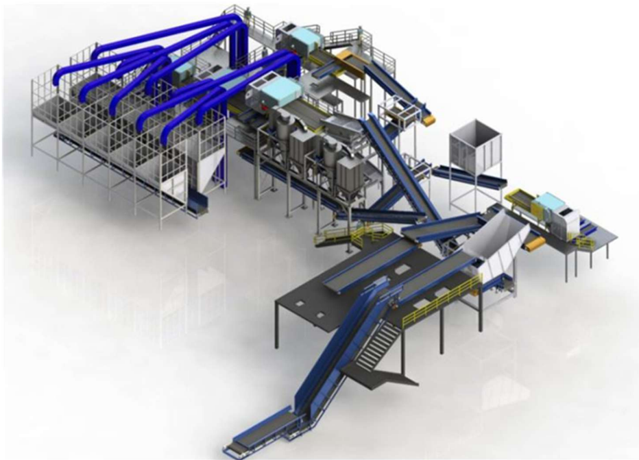
Figure 6 – Full-Scale Secondary MRF (Example Only)
